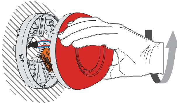
Wall mounting of FDS221 alarm sounder in an FDB221 detector base
