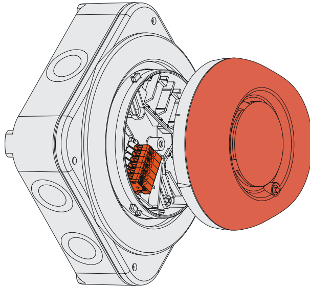
Wall mounting of FDS221 alarm sounder with a base attachment humid FDB293 and a detector base FDB221
